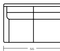
920-05-1L LEFT ARM LOVESEAT H36 W55 D37 INSIDE: H16 W49 D22 SEAT H: 20 ARM H: 24
