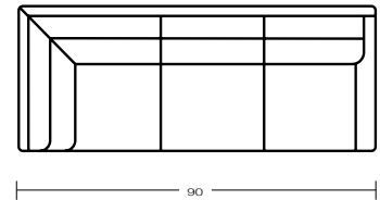
920-00R RIGHT ARM CORNER SOFA H36 W90 D37 INSIDE: H16 W74 D22 SEAT H: 20 ARM H: 24
