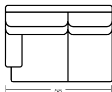
2565-1L LEFT ARM LOVESEAT OR 2565-1R RIGHT ARM LOVESEAT H39 W58 D41 INSIDE: H19 W49 D22 SEAT H: 20 ARM H: 24
